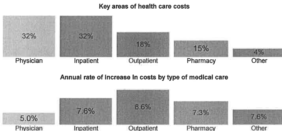
This chart shows how annual trend rates will fluctuate based on the percentage of services used within each component by the insured population in any given year. Source: percentages in both graphs are based on analysis of 2012 Milliman Medical Index, May 2012, pages 2-3.
