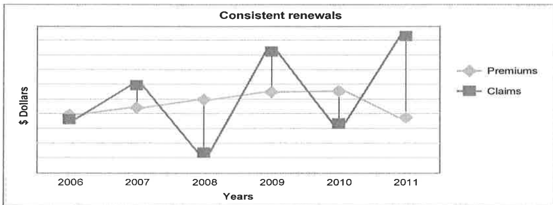
This chart shows the renewal premiums and claims experience of an actual Sun Life customer with 600 lives.
